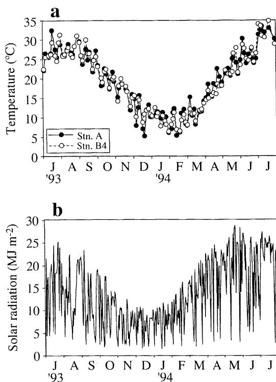
Figs. 2a and b. Low-tide water temperature (a) recorded during each sampling occasion at Stns. A and B4 and daily solar radiation (b) obtained from the Takamatsu Meteorological Agency station where the intertidal flat is located.
