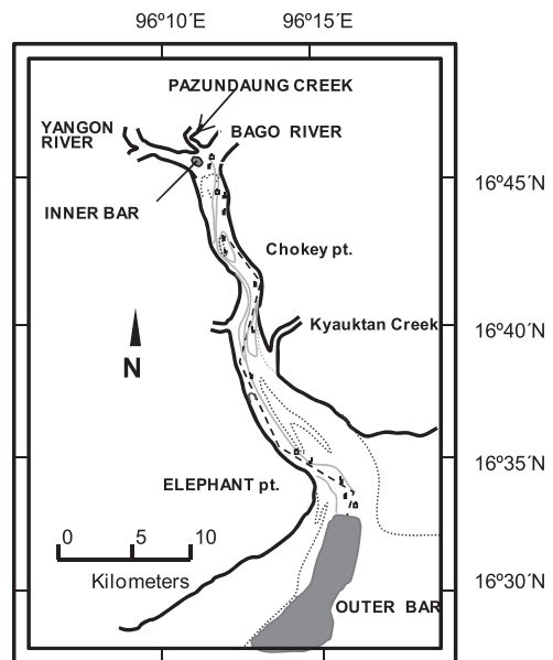
Fig. 1. Locations of Yangon River and Estuary and the two sand bars, Inner Bar and Outer Bar
